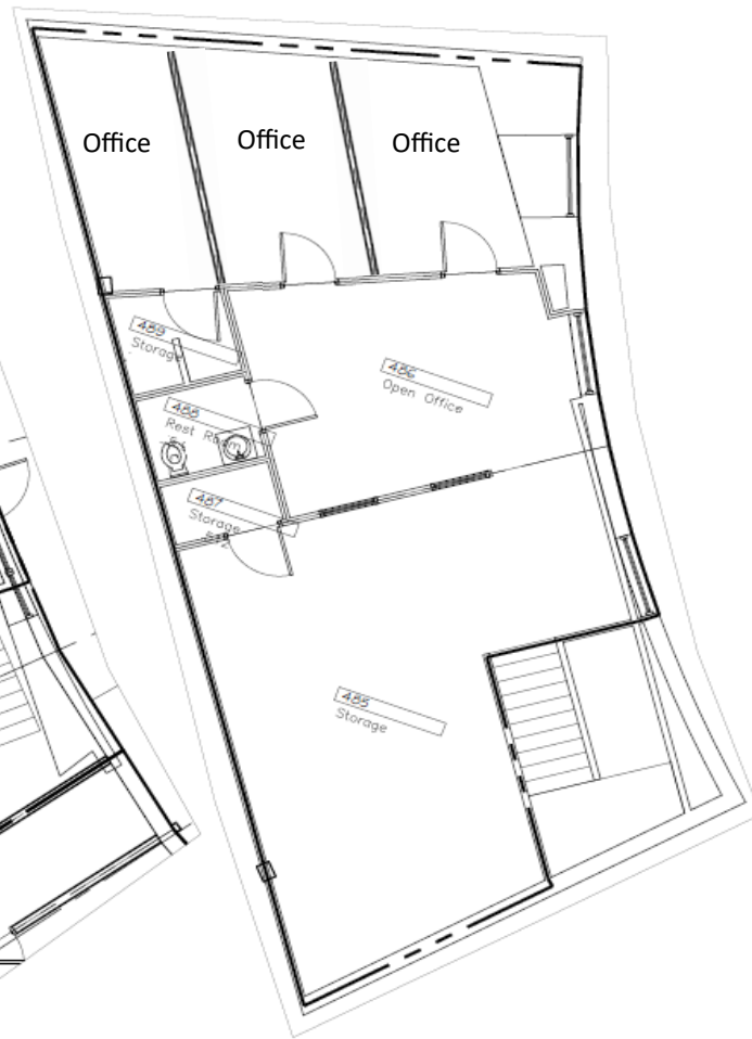
Ground Floor Plan Scale: 1/8" = 1'-0"
